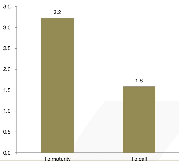
Duration, years
